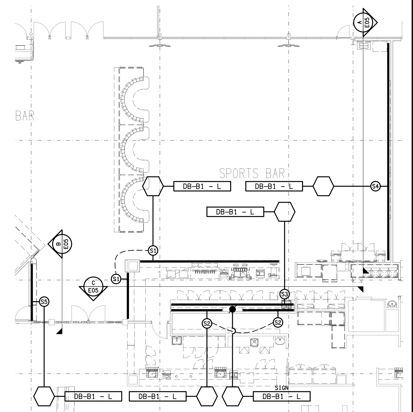
PART PLAN JOINERY LIGHTING SCALE 1:100
